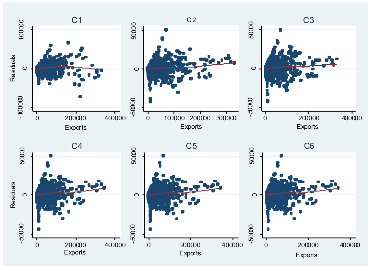
Figure 5. Residuals versus observed values
